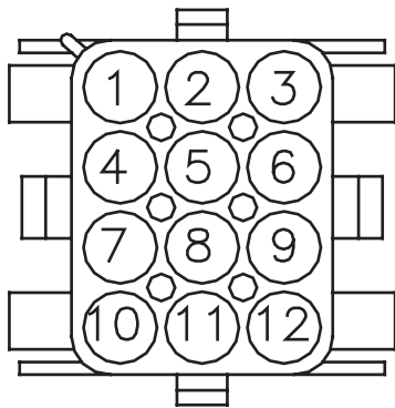
View from cable side
